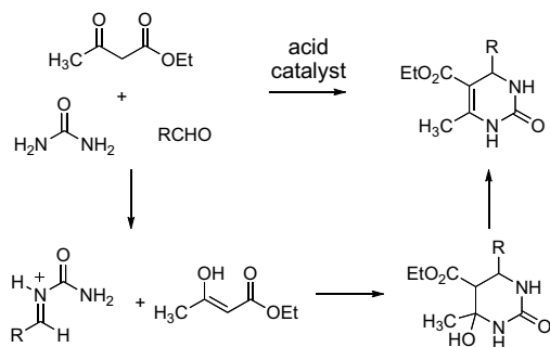
Scheme 1. Biginelli reaction.
